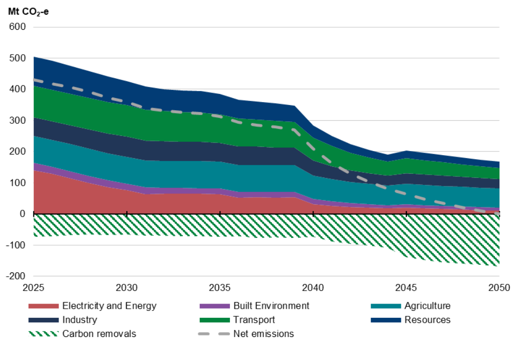
Chart A.3: Projected emissions reductions, by Sector, Disorderly Transition Scenario
