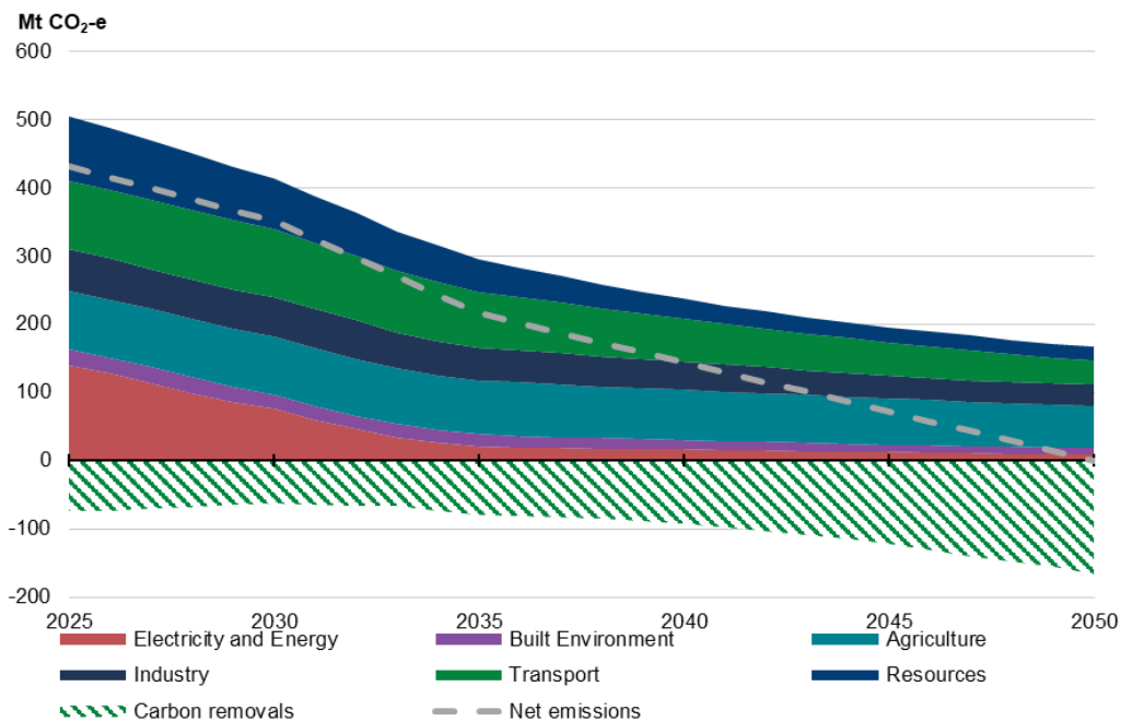
Chart A.1: Projected emissions reductions, by Sector, Baseline Scenario
